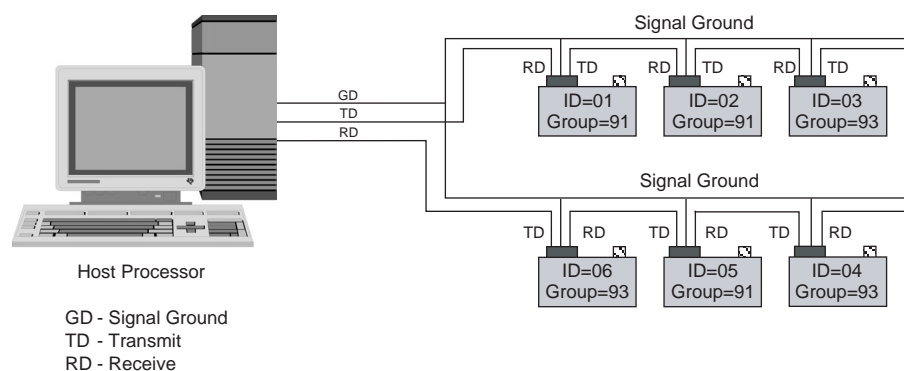
Figure 4.12—HPB RS-232 Ring Network
