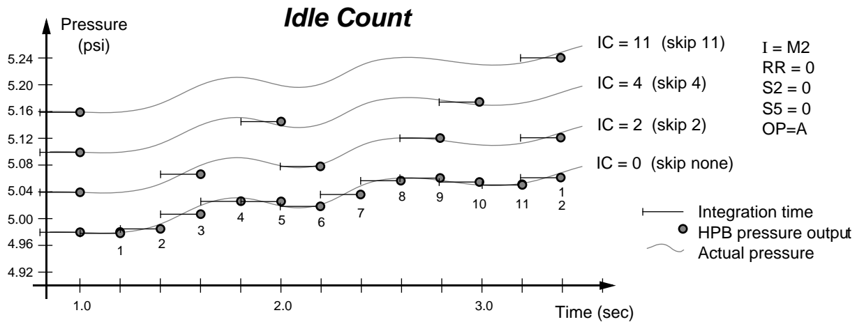
Figure 4.10—Idle Count (IC) Command Example
