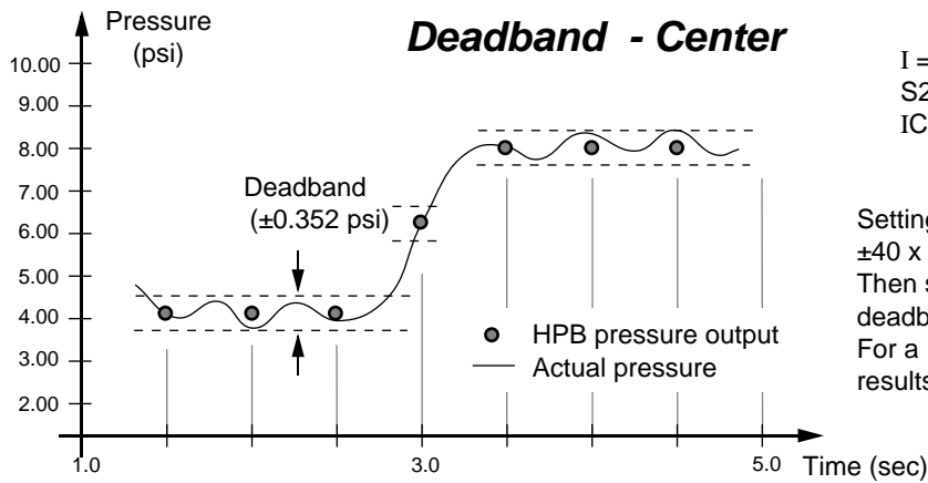
Figure 4.9a—Deadband and Sensitivity (DS) Command Examples
