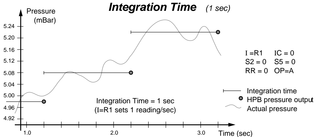
Figure 4.6—Integration (I=) Command, Example 2
