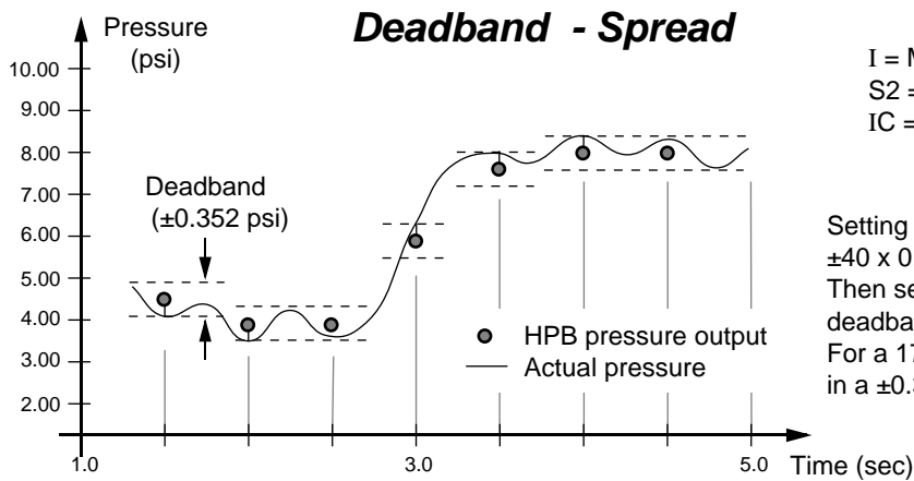
Figure 4.9b—Deadband and Sensitivity (DS) Command Examples
