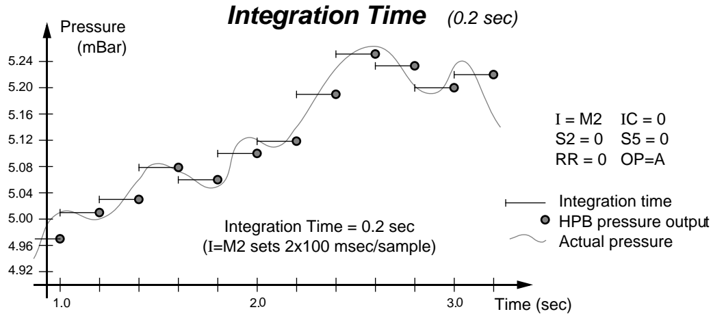
Figure 4.5—Integration (I=) Command, Example 1
