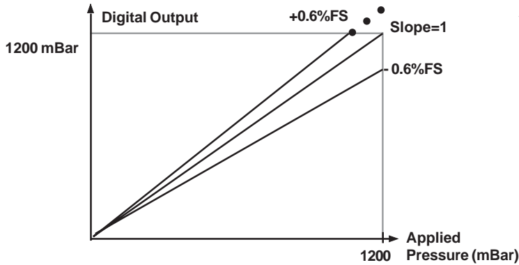
Figure 4.3—Custom Slope (X=) Options
