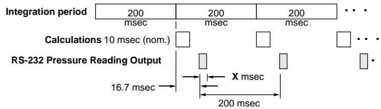
Figure 7.2—Default Continuous Pressure Reading Timing Diagram
