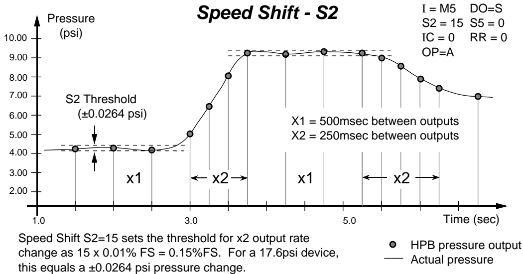
Figure 4.7—S2 Speed Shift Command Example
