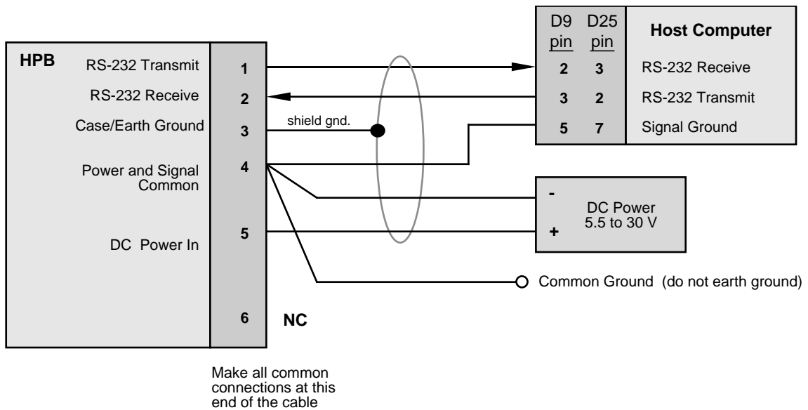
Figure 6.1—HPB and HPB-CE Electrical Connector Pin Assignments
