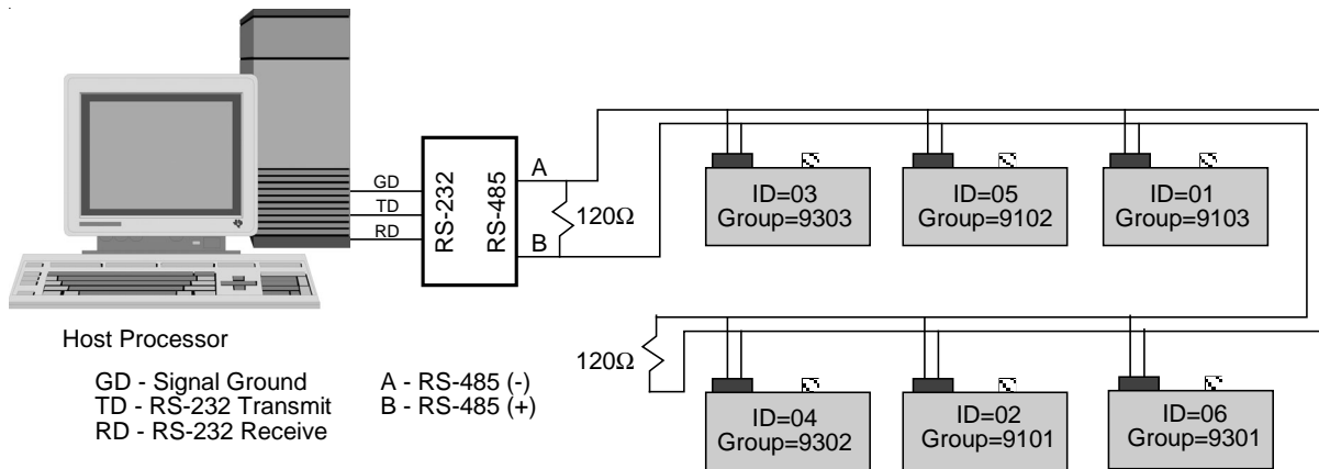
Figure 4.13—HPB RS-485 Multidrop Network
