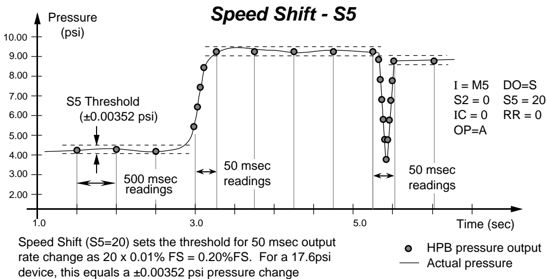
Figure 4.8—S5 Speed Shift Command Example
